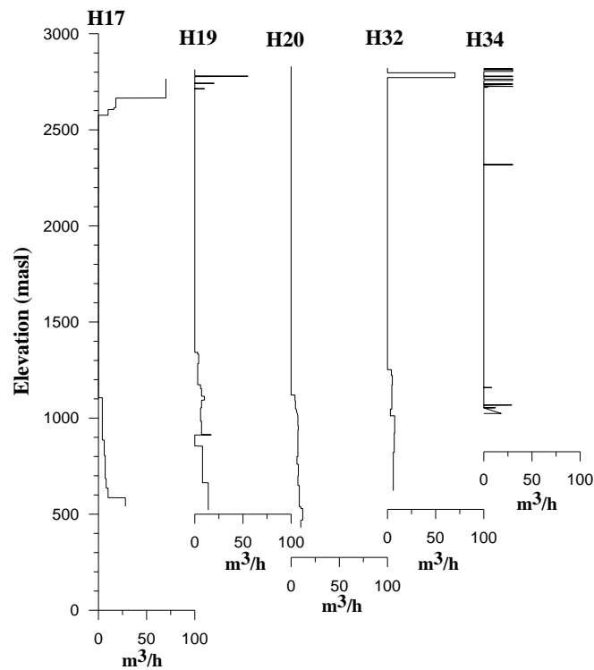
Fig. 12. Circulation losses profiles, during drilling of wells located in the sector bounded by “Los Pájaros” and “Las Víboras” faults
