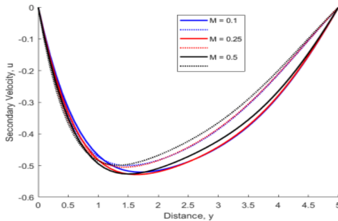
Fig. 18. Secondary velocity profiles for different values of M=0.1, 0.25, and 0.5
