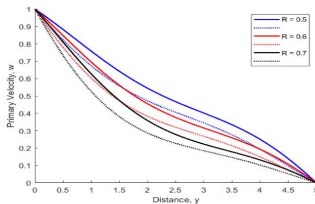
Fig. 8. Primary velocity profiles of varying R, R=0.5, 0.6, and 0.7
