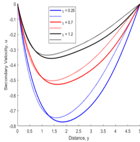
Fig. 15. Secondary velocity profiles for different values of \chi , \chi=0.25, 0.7, and 1.2
